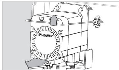
Quick-change pump
