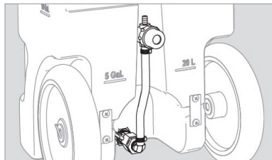
In-line strainer to protect pump from debris
