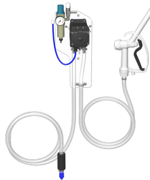
Chemical Transfer Unit For Up To Four Products CTX
