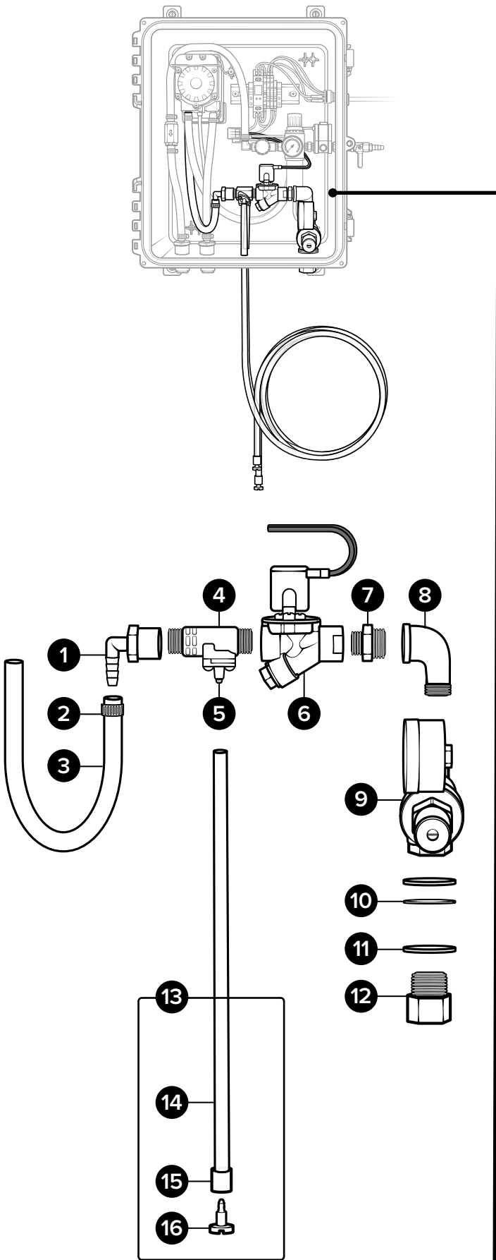
WRGA-FCV-24VDC-WC-RH
